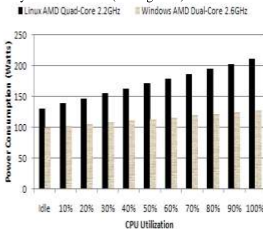
Fig 3: Power consumption under different workloads.
