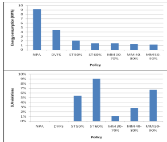
Fig 7: comparison of diff policies under different workloads with respect to cpu utilisation
