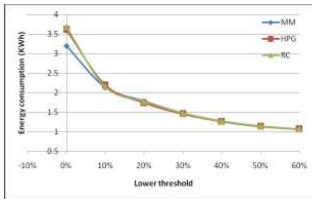
Fig 5:energy consumption of different policies
