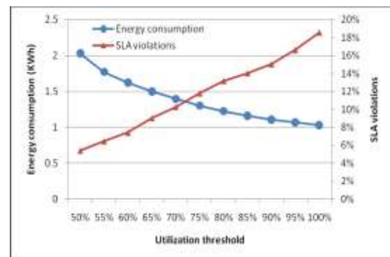
Fig 4:simulation results of ST policy
