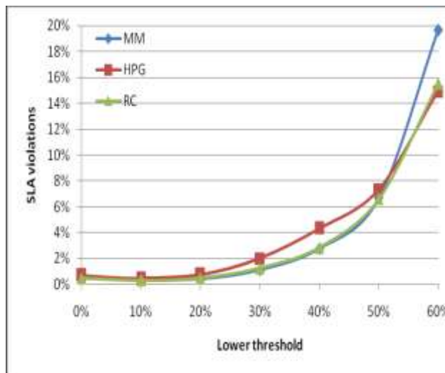
Fig6:SLA violations of different policies under different thresholds Comparison with respect to CPU utilisation
